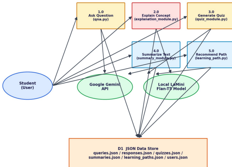
EduGenie - Data Flow Diagram (Level 1)
